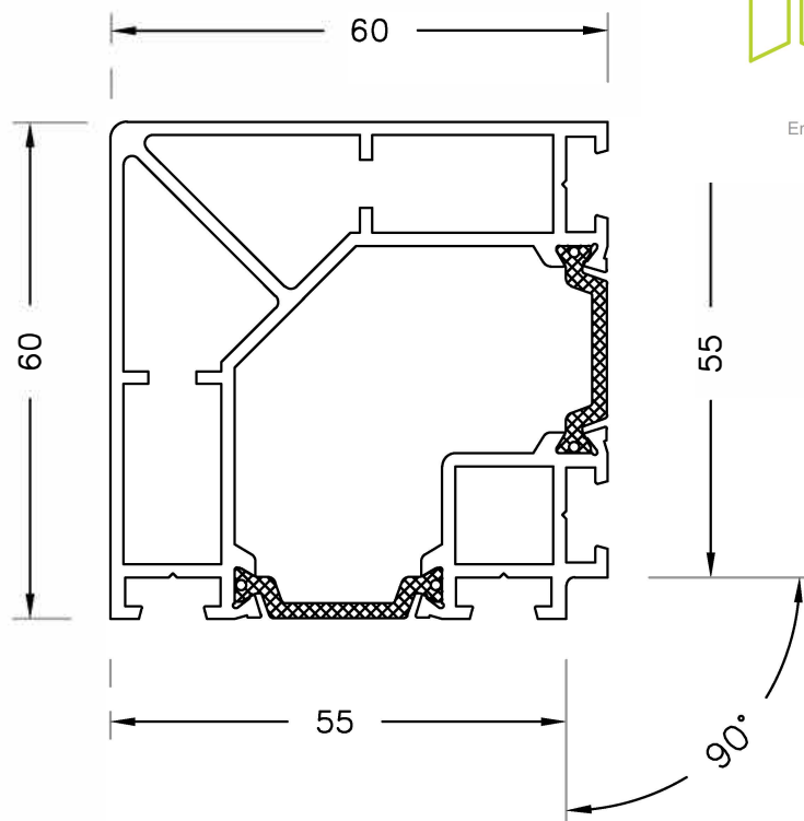
90° Post
