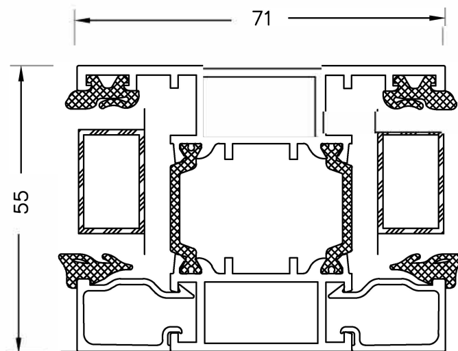
Transom / Mullion
