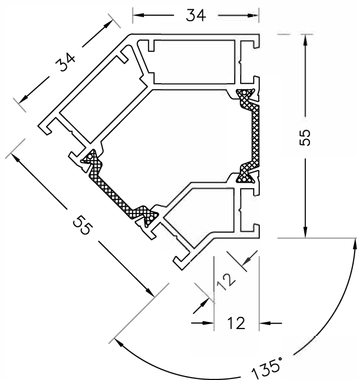
135° Post
