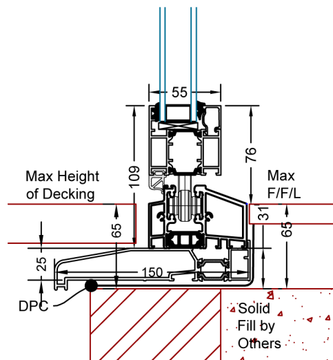
SF55 Low Level Open Out With Sill
