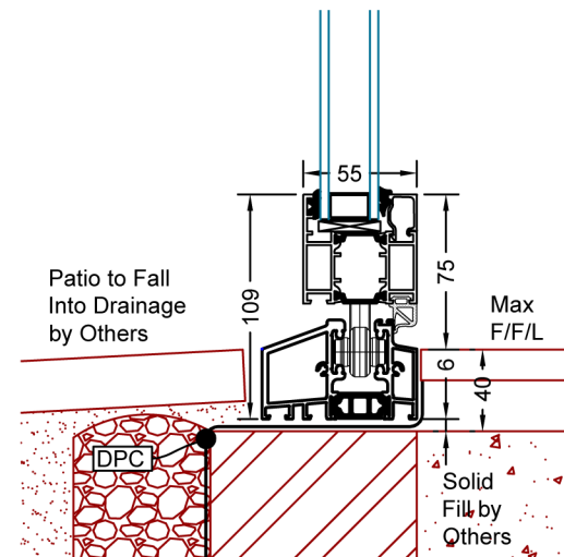
SF55 Low Level Open In Width Sill
