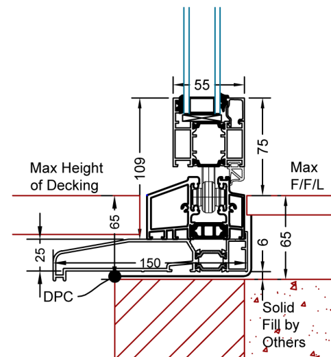
SF55 Low Level Open In Width Sill
