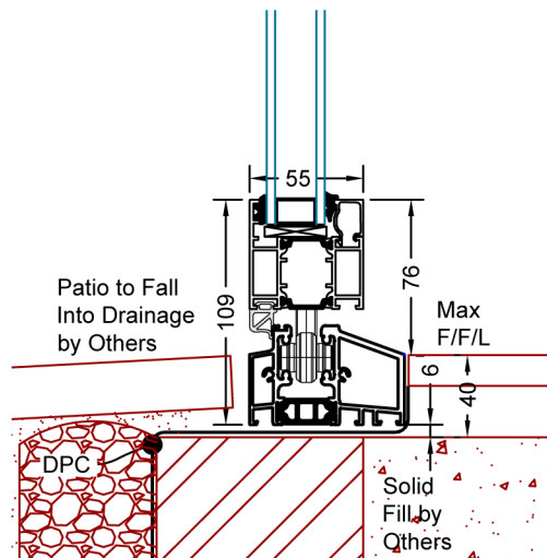
SF55 Low Level Open Out With Sill
